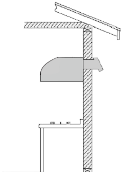
REAR VENTING
