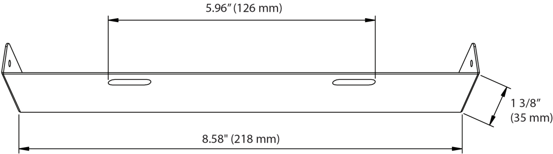
Upper Chimney Bracket.
