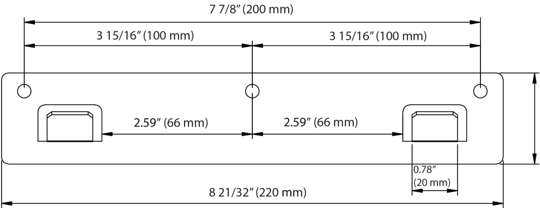
Mounting Bracket Hook
