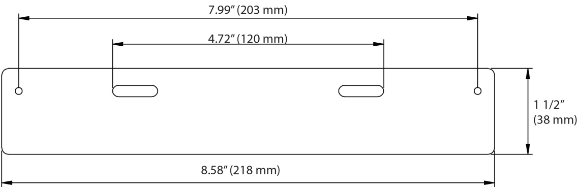
Lower Chimney Bracket
